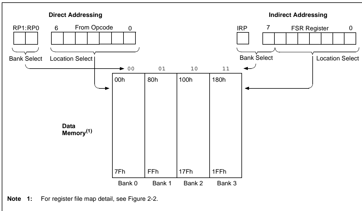
FIGURE 2-5: DIRECT/INDIRECT ADDRESSING
